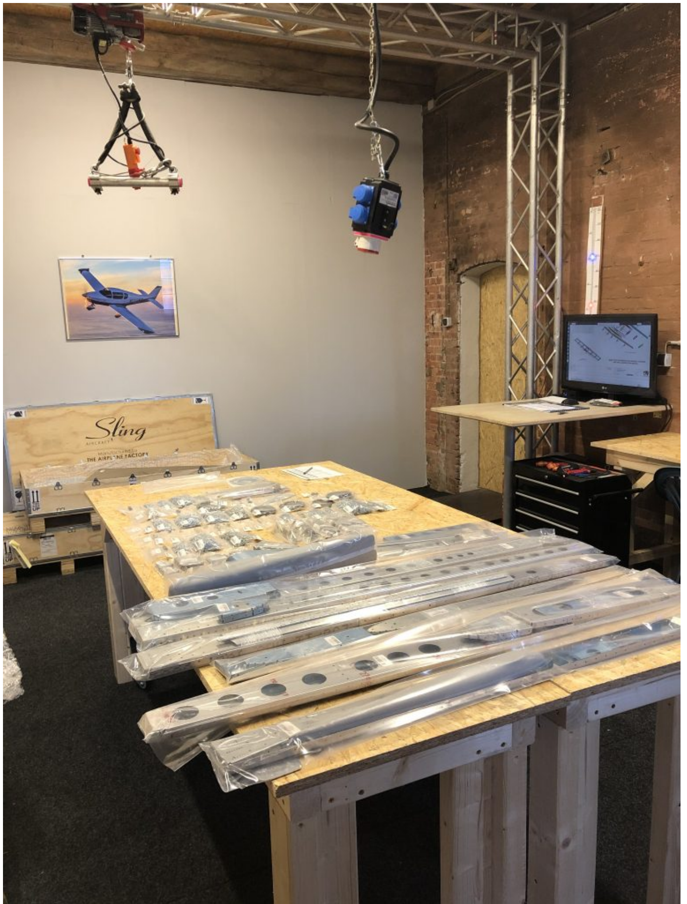
inventory the empennage kit
